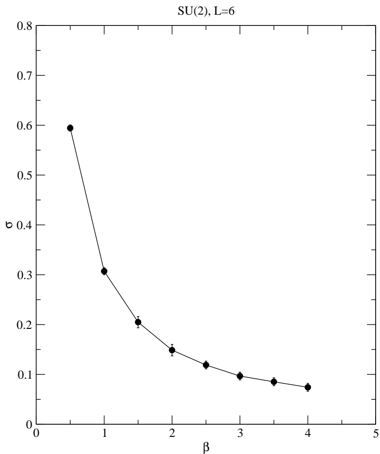
Figure 8: String tension for SU(2) and L = 6 .
