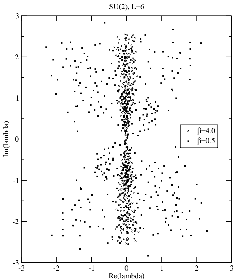
Figure 6: Eigenvalue spectrum for SU(2) theory at L = 6 .
