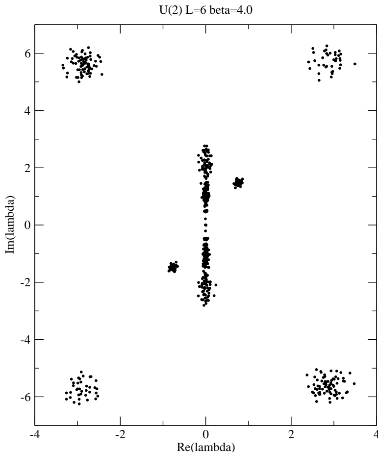
Figure 4: Eigenvalue spectrum for U(2) theory at \beta = 4.0 .
