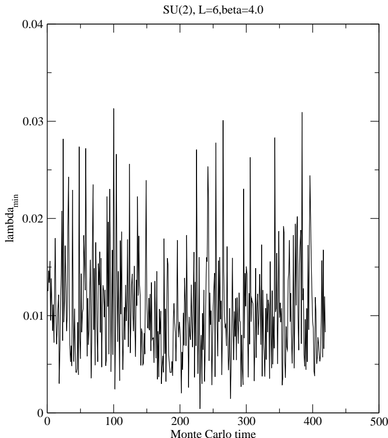
Figure 7: Minimum eigenvalue for SU(2) theory at L = 6 .
